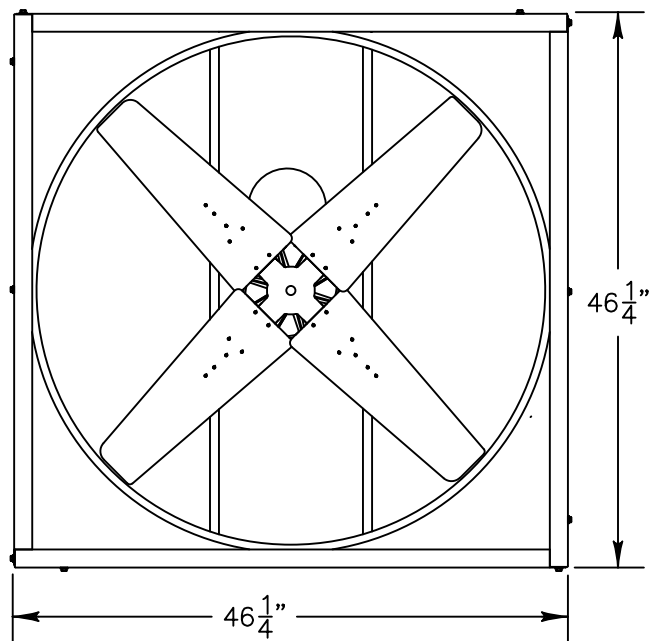
DISCHARGE VIEW
