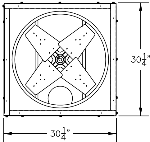
DISCHARGE VIEW
