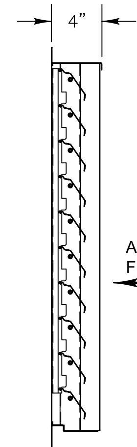
SIDE SECT VIEW
